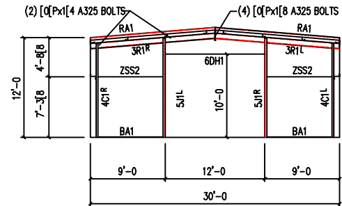
ENDWALL FRAMING @ COL. LINE "1"
