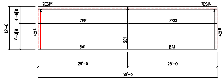
SIDEWALL FRAMING @ COL. LINE "B"
