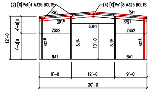
ENDWALL FRAMING @ COL. LINE "3"
