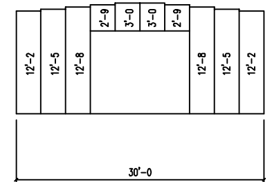
ENDWALL SHEETING @ COL. LINE "1"
