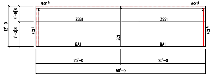
SIDEWALL FRAMING @ COL. LINE "A"
