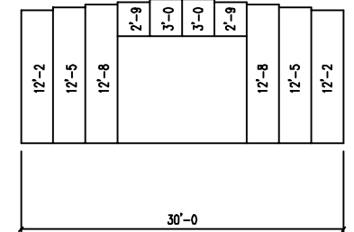
ENDWALL SHEETING @ COL. LINE "3"
